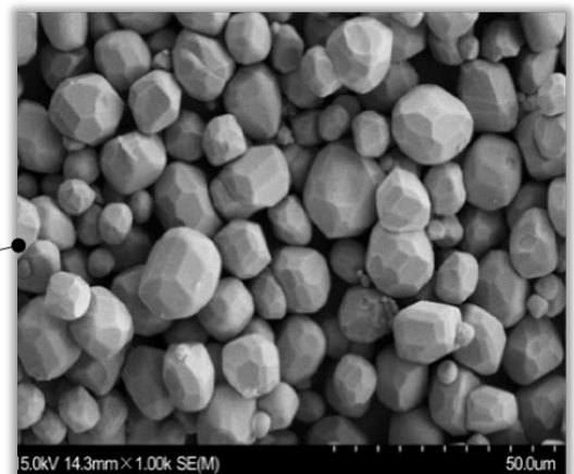
SEM of YAG (Yttrium-Aluminate-Garnet)
