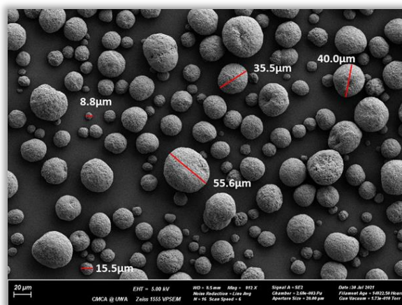
Scanning Electron Microscope (SEM) image of spherical, low surface area boehmite powder
